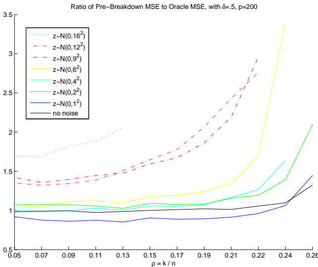
Fig. 10. Ratio of median Forward Stepwise MSE to the median oracle MSE. The number of variables is fixed at 200, the number of observations at 100, i.e. \delta = \frac{n}{p} = .5 , and the median was taken over 1000 replications. The error rates were truncated at the maximum first difference, to isolate the region in which Forward Stepwise does recover the underlying model correctly. At higher noise levels, the breakdown point occurs at lower sparsity levels, i.e. the model must be more sparse for Forward Stepwise to recover it with small error. The errors increase more for Forward Stepwise with increasing noise levels, than for the oracle MSE.
