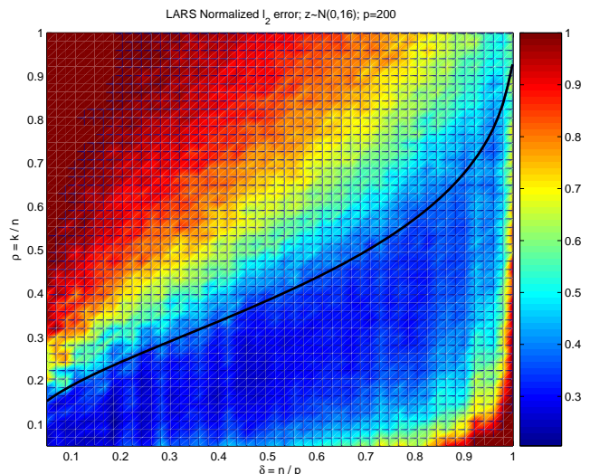
Fig. 3. This diagram displays the median error rates when the LARS Algorithm [7] is used to recover the underlying sparse model, with the number of variables, p , fixed at 200. The algorithm does not find the correct model well above the threshold, and seems to have trouble when there are as many predictors as observations. Each color indicates a different median normalized l_2 error of the coefficients \frac{\|\hat{\beta} - \beta\|_2}{\|\beta\|_2} over 30 realizations.
