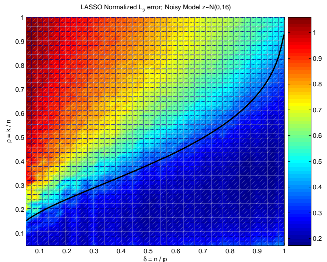
Fig. 2. Phase transition diagram when the sparse model is recovered using the LASSO Algorithm [8], where the number of variables, p , is fixed at 200. The theoretical phase transition curve from Fig 1 has been superimposed. The dark blue area, below the curve, indicates where the algorithm recovered the underlying model with near zero error, but above the curve in the colored area, the algorithm was unable to recover the correct model. As you proceed further above the curve, the ability of the algorithm to recover the model progressively drops. As with the theoretical phase transition diagram in Fig 1, along the x-axis the level of underdeterminedness decreases, and along the y-axis the level of sparsity of the underlying model increases. Each color indicates a different median normalized l_2 error of the coefficients \frac{\|\hat{\beta} - \beta\|_2}{\|\beta\|_2} over 30 realizations.
